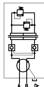
Hydraulic circuit Diagram
