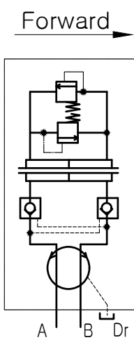
Hydraulic circuit Diagram
