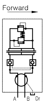
Hydraulic circuit Diagram
